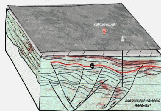
Present day structural model - Traps
