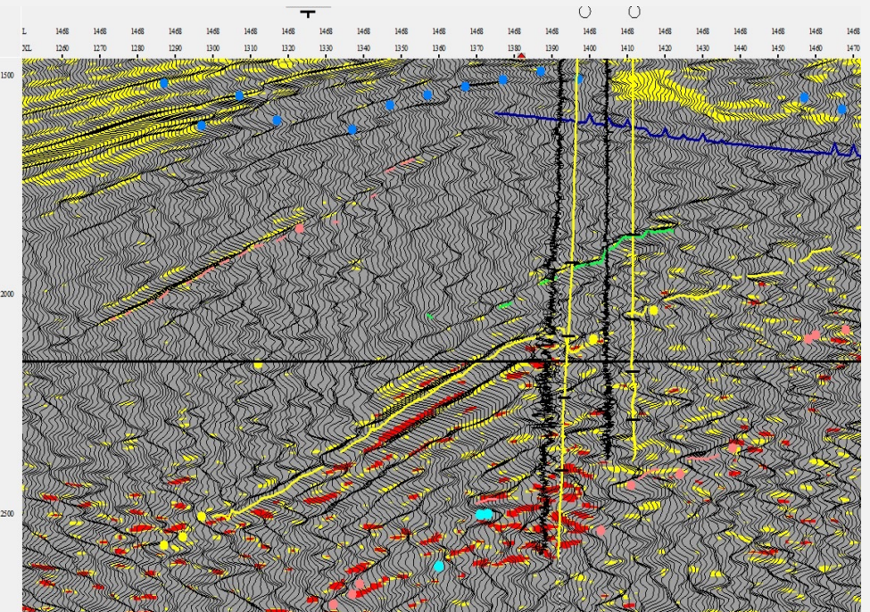
Deterministic Pre-Stack Seismic Inversion Volume
